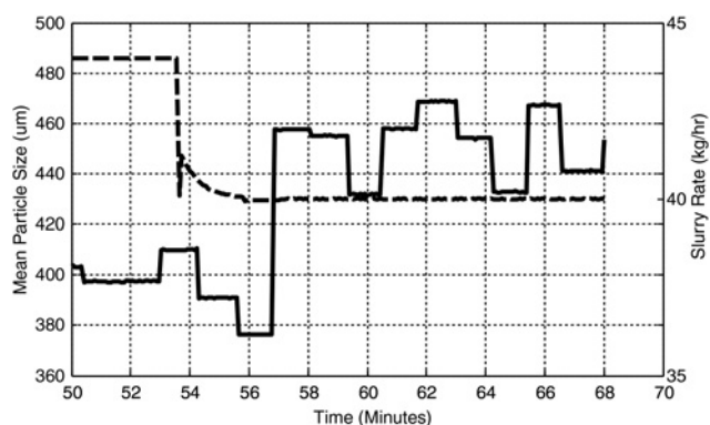
Fig. 7 Positive change in MPS to a decrease in slurry rate, '—' MPS, '---' slurry rate (pump speed prediction)
