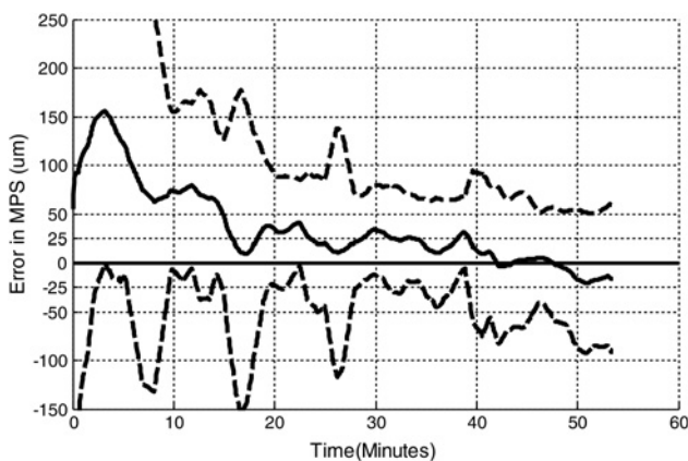
Fig. 4 Average error in MPS for 15 batches using ratio control \pm \sigma , '—' average, '- -' \pm \sigma
