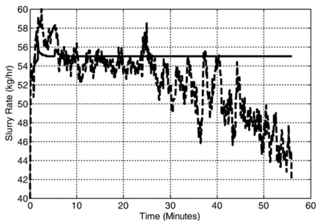
Fig. 6 Changes in slurry rate mass flow at a constant pump speed, '---' empirical pump correlation, '—' load cell measurement
