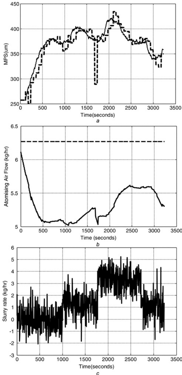
Fig. 3 Simulation of the MPS, the change in the atomising air-flow rate to control the MPS and the disturbance produced from the slurry rate a Simulated MPS controlled at 375 μm and subject to disturbances, ‘—’MPS, ‘- - -’ b Simulated change in atomising air-flow to control MPS, ‘—’ air-flow, ‘- - -’ initial value c Simulated change in slurry rate with additional noise from steady state
