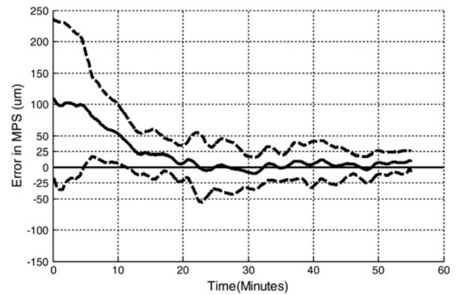
Fig. 5 Average error in MPS for 15 batches using cascade control \pm \sigma , '- -' average, '—' \pm \sigma
