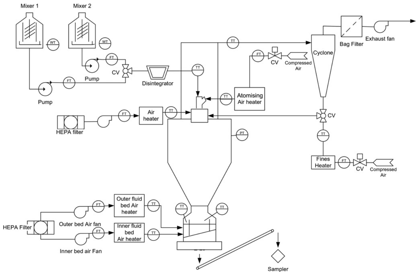
Fig. 1 Piping and instrumentation diagram of mixed flow spray dryer
