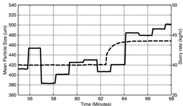
Fig. 8 Positive change in MPS to an increase in slurry rate, '—' MPS, '---' slurry rate (pump speed prediction)
